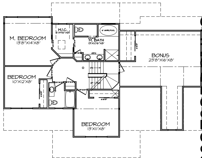
SECOND FLOOR PLAN A-5
