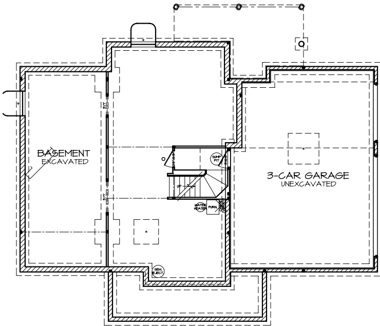
FOUNDATION PLAN A-3
